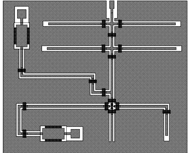
Figure 1: Layout of 26 GHz HBT coplanar oscillator.
