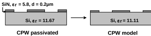
Figure 3: Implementation of the passivation layer in the CPW model.
